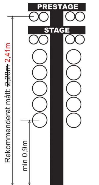
Figur 4. Startgranen
